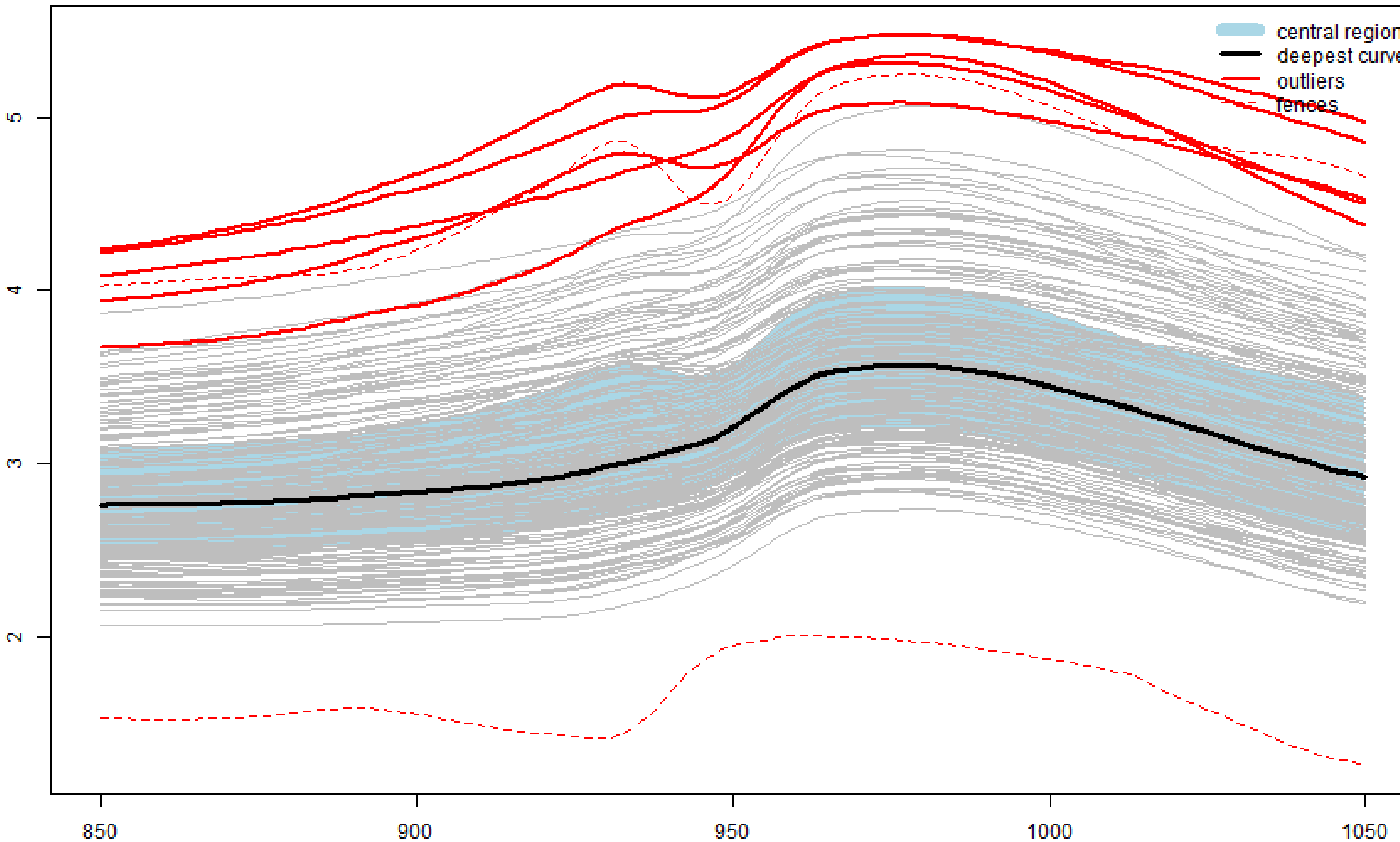
Tecator Functional Boxplot
